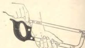
To tension blade
