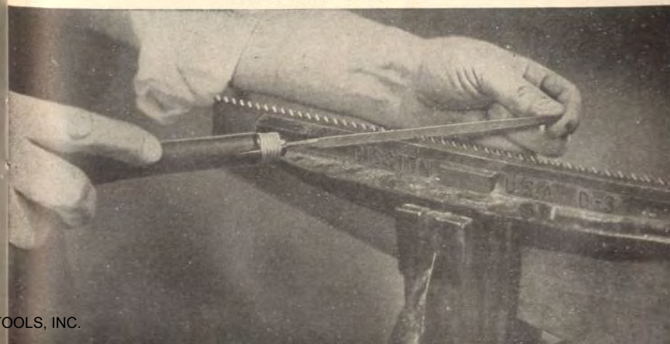
POSITION of file for beveling teeth
