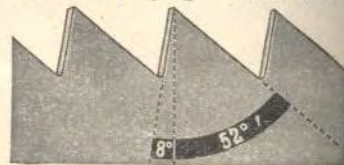
Side view of rip teeth (enlarged)
