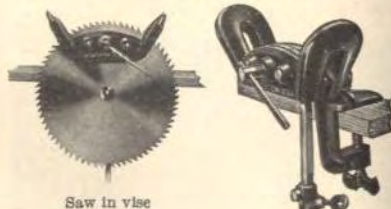
Disston Circular Saw Filing Vise No. 7
