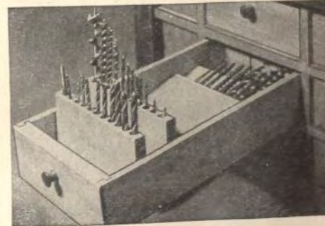
A SIMPLE method of keeping bits and drills in order. Wood blocks drilled with holes are hinged to bottom of drawer. They lie flat when drawer is closed.
